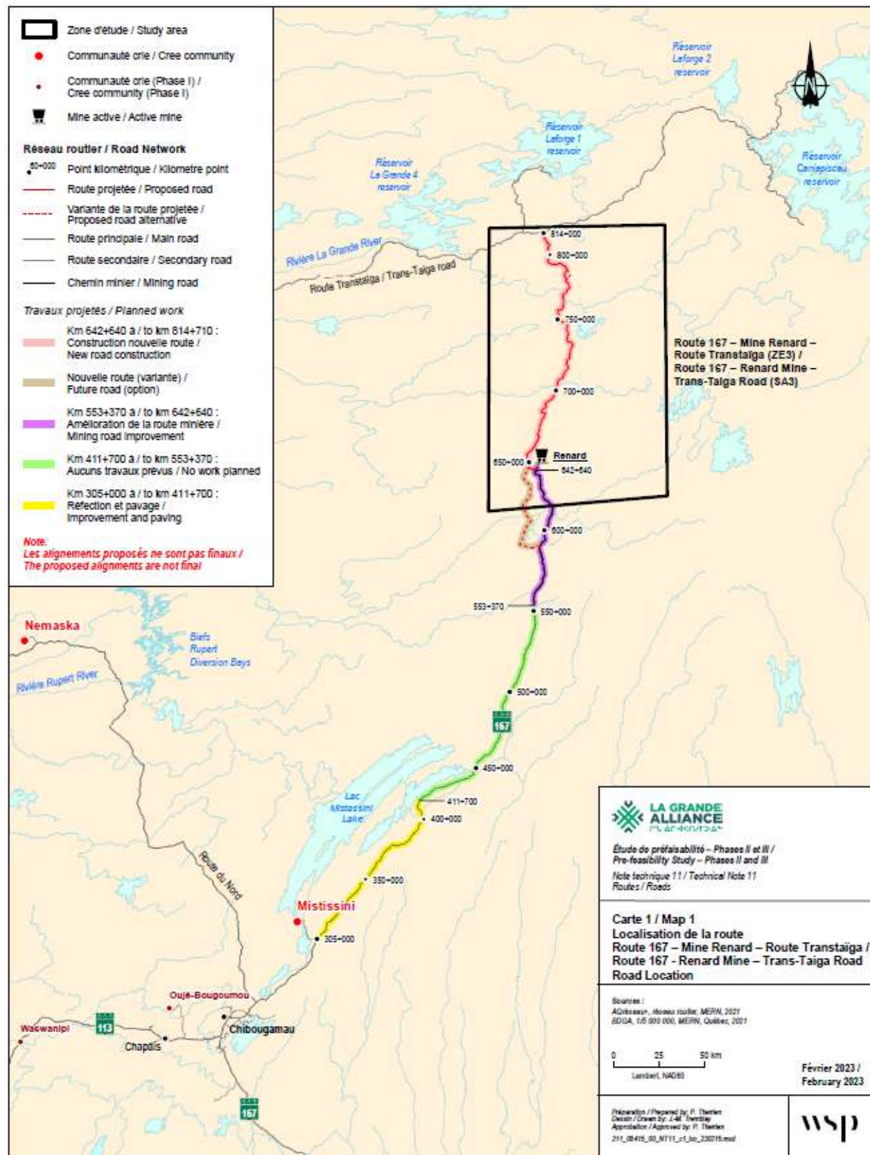
Figure 5-1 Route 167: Upgrade & Extension to Trans-Taiga – Proposed alignment
