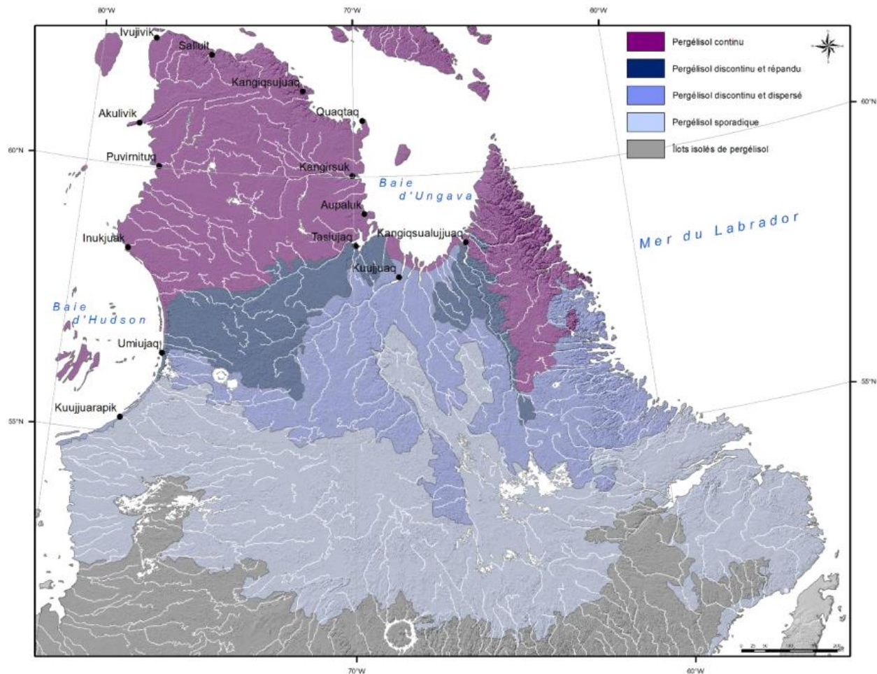
Figure 4-1 Distribution of permafrost in northern Quebec (Modified from Allard et al., 2012)
